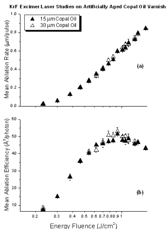
Figure 3.3.2.6 Laser ablation rate (a) and efficiency (b) at 248 nm against fluence for artificially aged copal oil varnish films.
