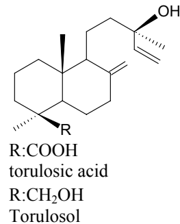
Figures 2.4.5 The characteristic abietane, pimarane and labdane type diterpenoid molecules of the conifer resins.
