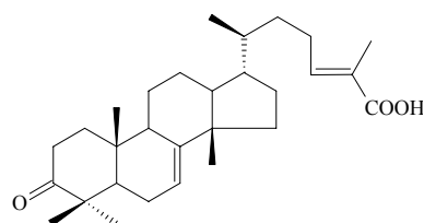
(iso)masticdienonic acid
