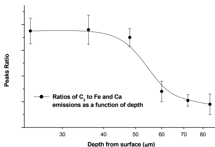
Figure 1.4.4 Ratios of C_2 to Fe and Ca emissions detected with LIBS as a function of ablated depth.
