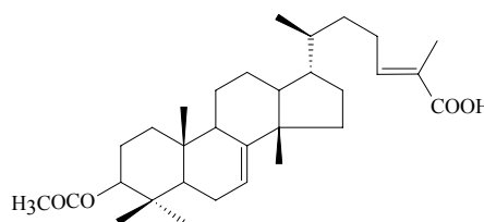
3-O-acetyl-3-epi(iso)masticdienolic acid
